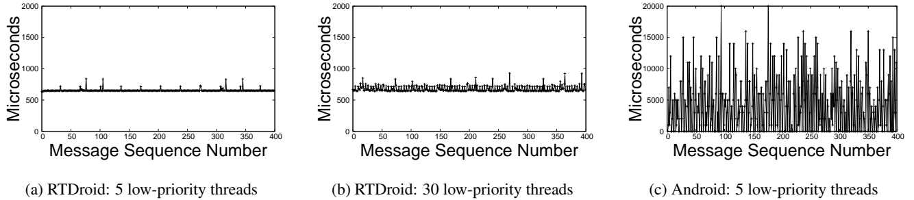
Figure 10: The observed raw latency of Looper and Handler on LEON3 Please note graph (c) has a different Y-axis.
