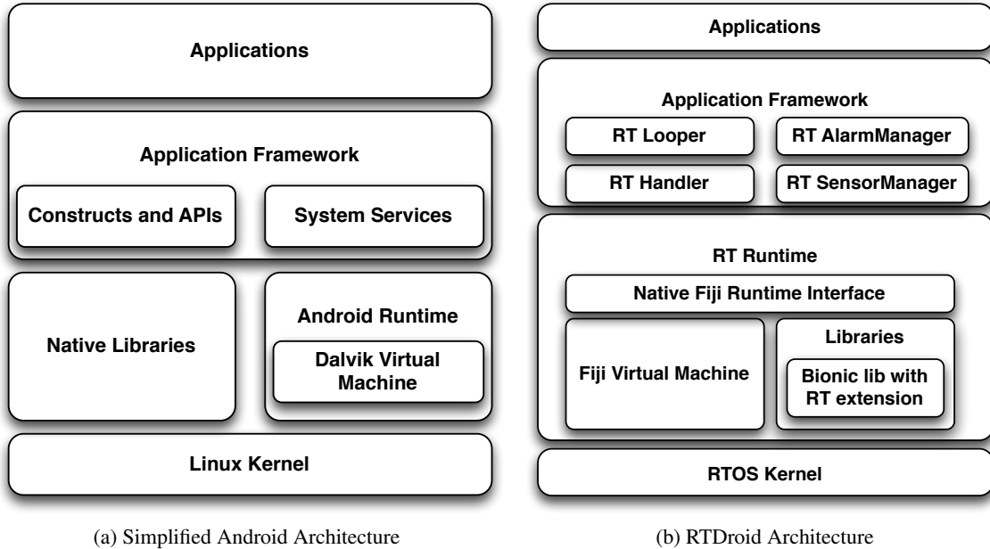
Figure 1: Comparison of Simplified Android and RTDroid Architectures
