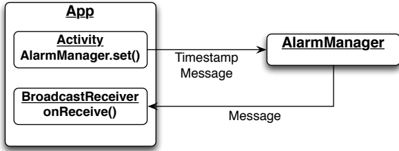
Figure 5: An Example Flow of AlarmManager. An application uses AlarmManager.set() to register an alarm. When the alarm triggers, the AlarmManager sends a message back to the application, and the application’s callback ( BroadcastReceiver.onReceive() in the example) gets executed.
