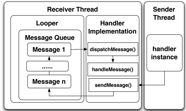
Figure 2: The Use of Looper and Handler
