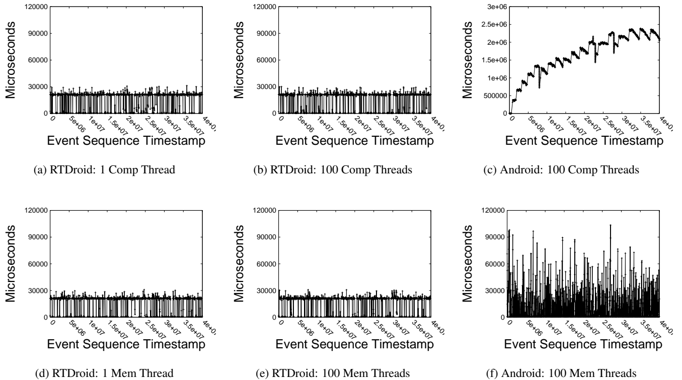
Figure 14: Memory and Computation stress test for the Fall Detection Application on Nexus S.
