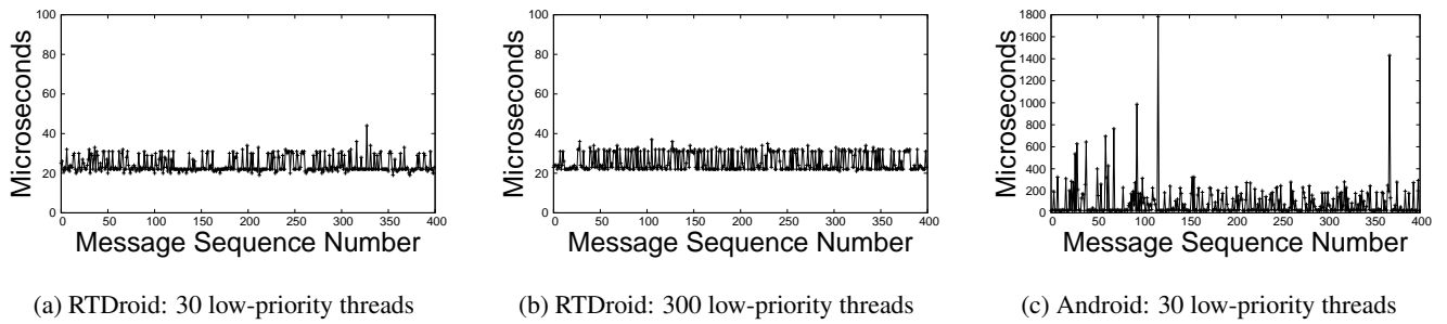
Figure 9: The observed raw latency of Looper and Handler on x86. Please note graph (c) has a different Y-axis.
