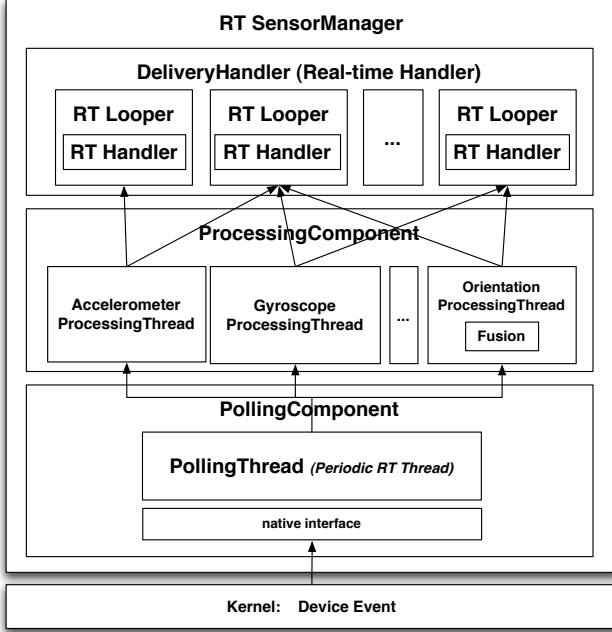
Figure 8: RTDroid Sensor Architecture
