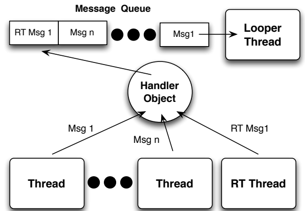
Figure 3: The thread in which the looper executes processes the messages sent through this handler object in the order in which they are received.
