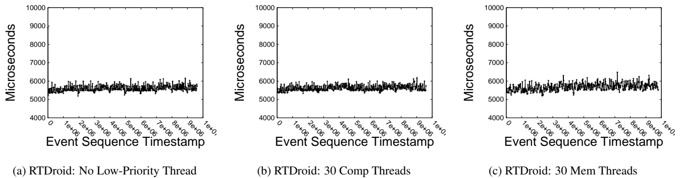
Figure 15: Memory and Computation stress test for the Fall Detection Application on LEON3.
