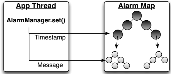
Figure 6: The Implementation of Alarm Execution on RTDroid. The tree colored black at the top maintains timestamps. The trees colored gray are per-timestamp trees maintaining actual alarm messages to be delivered.
