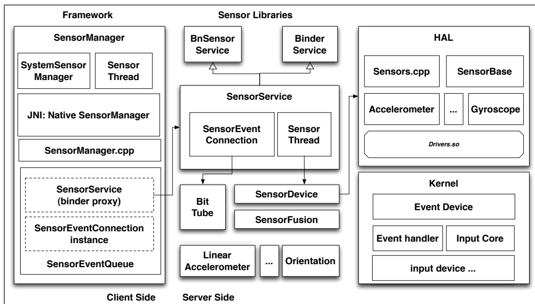
Figure 7: Android Sensor Architecture
