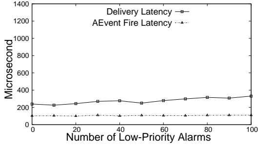
(a) RTDroid: Per Thread AEH
