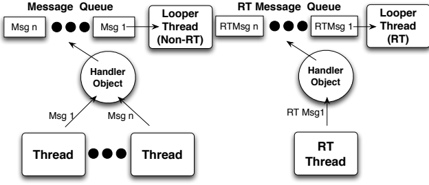
Figure 4: An Example of Looper and Handler in RTDroid. Each message has a priority and is stored in a priority queue. Processing of messages is also done by priority. The example shows one high-priority thread and multiple non-real-time threads.
