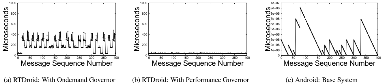
Figure 11: The observed raw latency of Looper and Handler on Nexus S. Please note graph (c) has a different Y-axis
