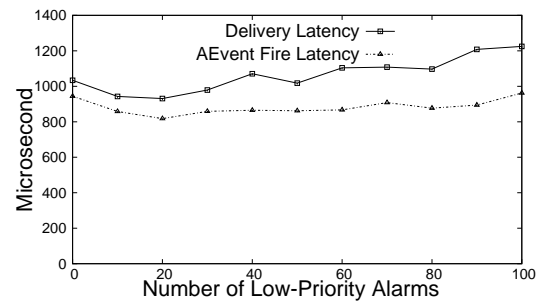
(b) RTDroid: Thread Pool AEH
